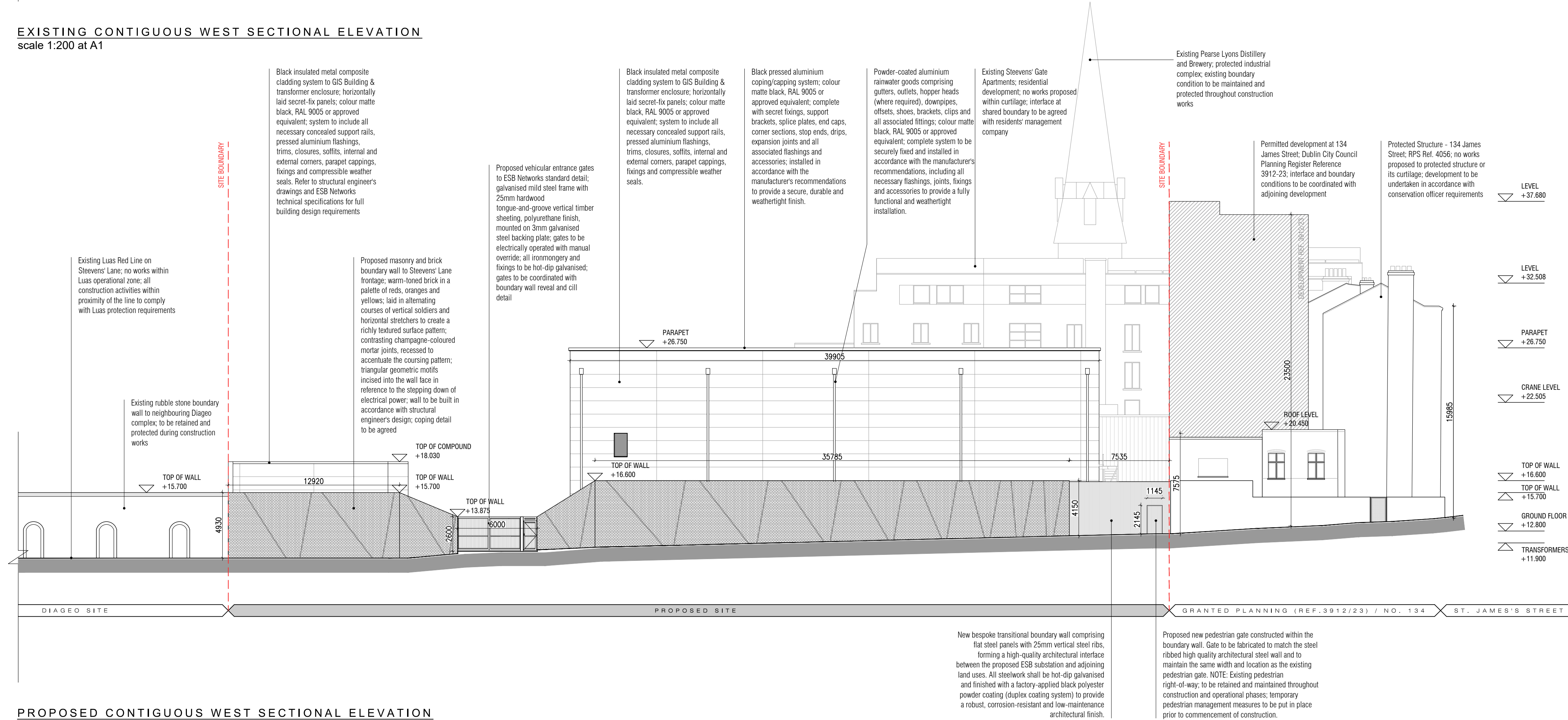
PROPOSED CONTIGUOUS WEST SECTIONAL ELEVATION scale 1:200 at A1
